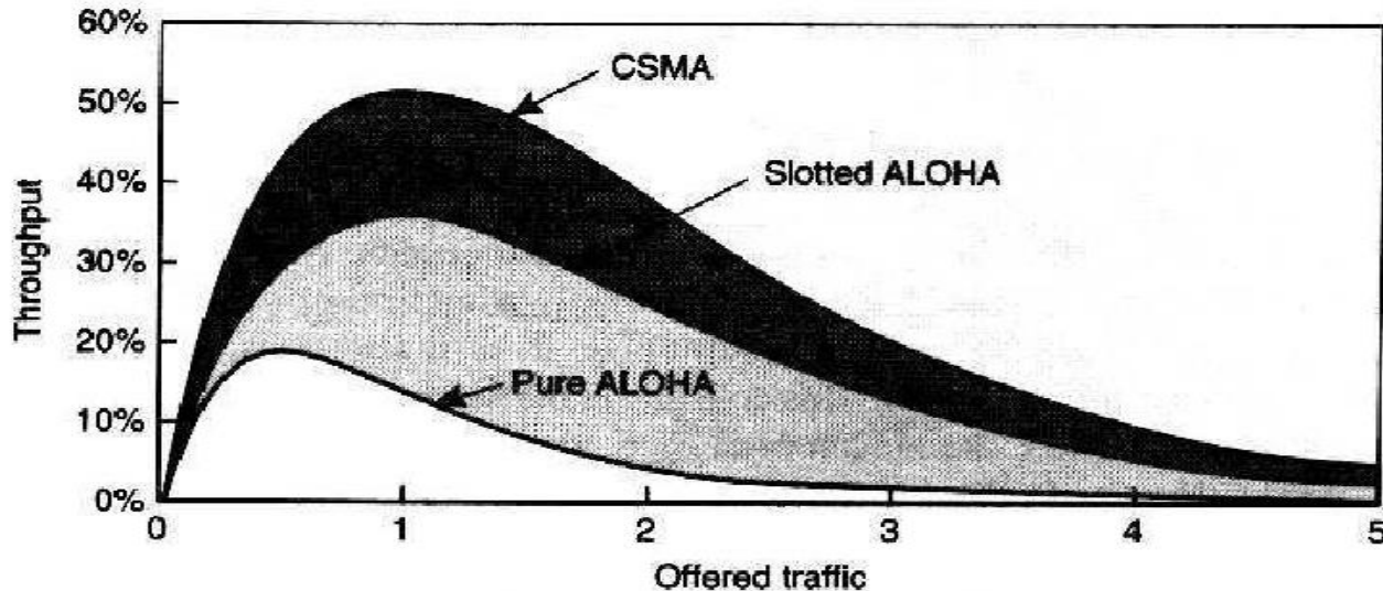
Figure 4.13 Performance of CSMA.
